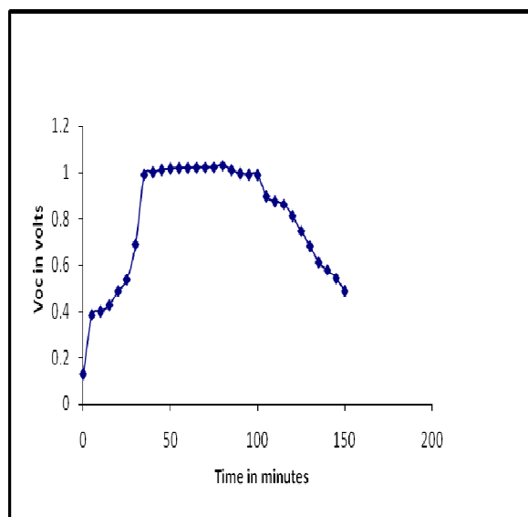
Fig. 6. Variation of open circuit voltage with time for Dairy waste based MFC with PANI coated graphite electrode.
