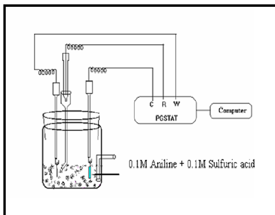
Fig. Electrochemical synthesis of polyaniline Substrate
