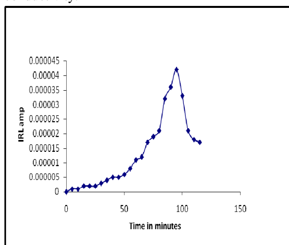
Fig.5. Variation of current with time for dairy waste based MFC with uncoated graphite electrode
