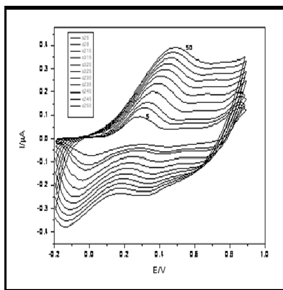
Fig. 2. Cyclic voltammetric scans recorded during polymerization. Scan number indicated in the figure
