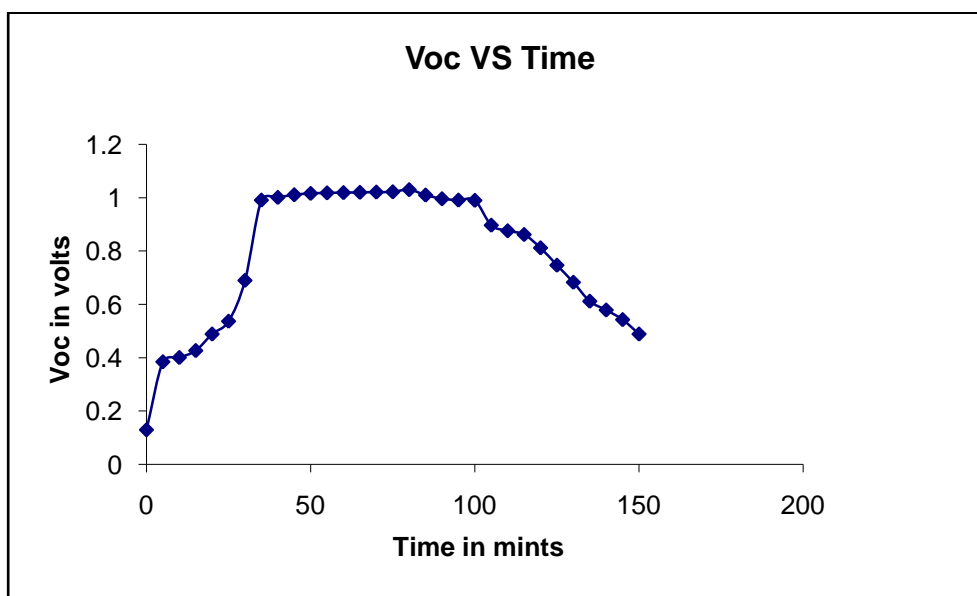
Fig. Variation of open circuit voltage with time for Dairy Waste based MFC with PANI coated graphite electrode.
