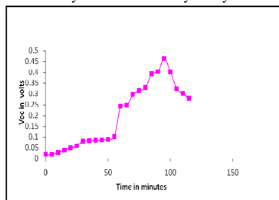
Fig. 3. Variation of open circuit voltage with time for Dairy waste based MFC with uncoated graphite electrode.
