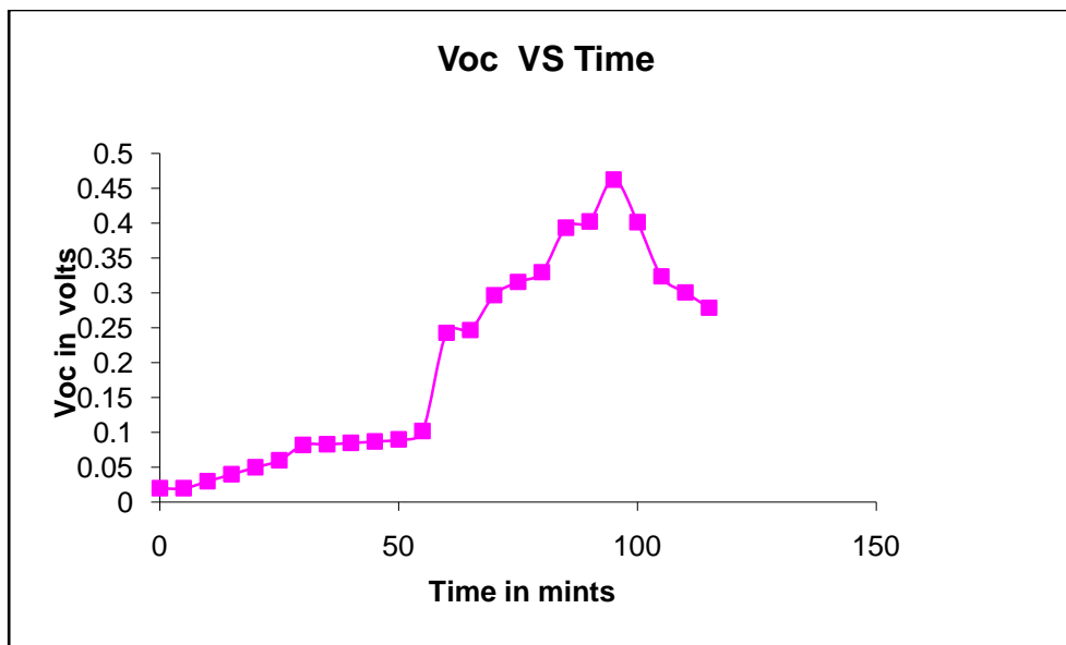
Fig. Variation of open circuit voltage with time for Dairy Waste based MFC with Un coated graphite electrode.
