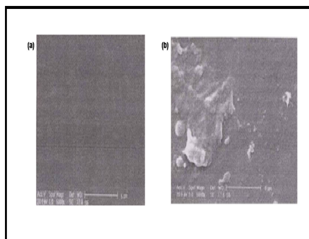
Fig . 4. 1 SEM images of graphite electrode a) before use b) after use
