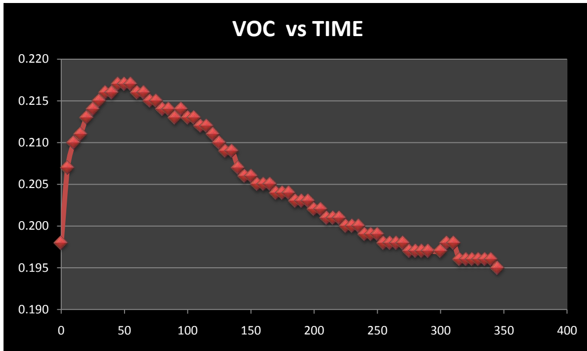
Fig .V OC Vs Time
